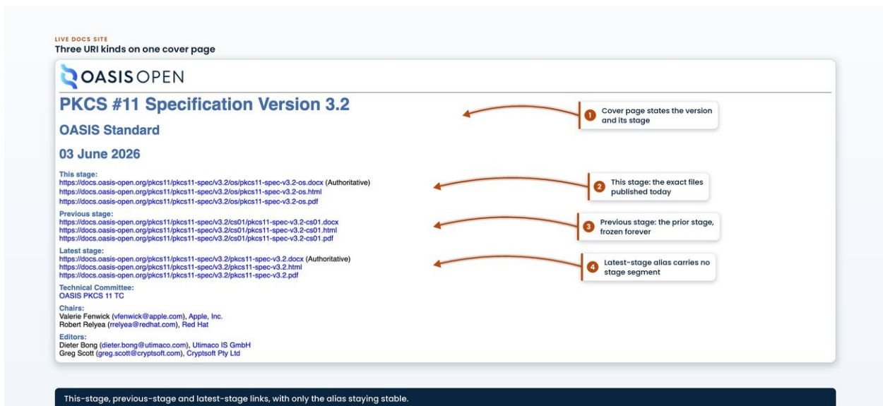
the published PKCS #11 Specification v3.2 cover page showing the This stage, Previous stage and Latest stage URI blocks, with the latest-stage alias carrying no stage segment
